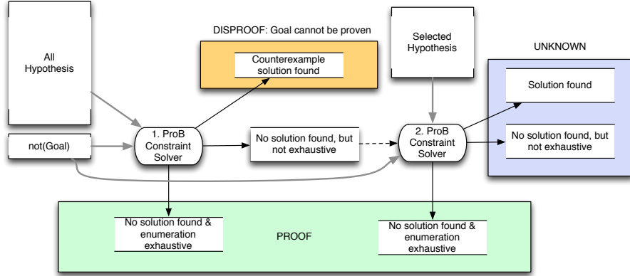
Fig. 1. Disproving Algorithm
