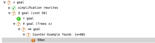
Fig. 1. Disproving Algorithm
