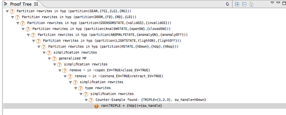
Fig. 3. Counter-Example for proof obligation of Landing Gear System by Andre et al.
